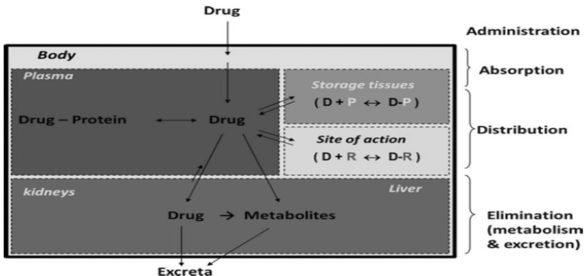
(Schematic diagram showing the various pharmacokinetic processes following administration of a drug. D drug, P protein, R receptor)
